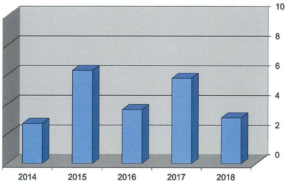
Fig. 2: SAIFI (lower is better)
